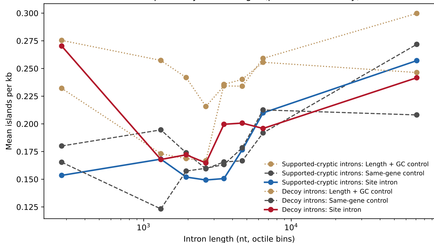
Islands per kb by intron length (phastCons 470way)
