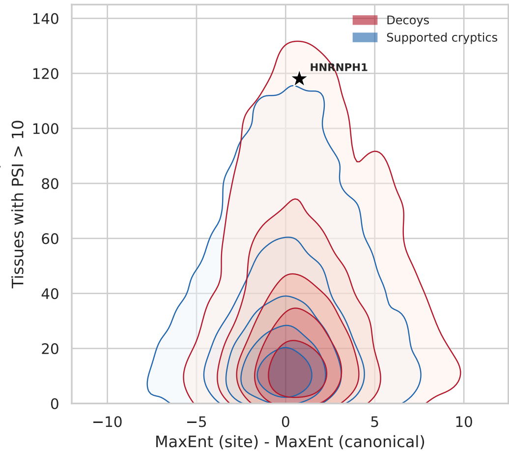
Overlay: decoys (red) and supported cryptics (blue), each as % of its class
