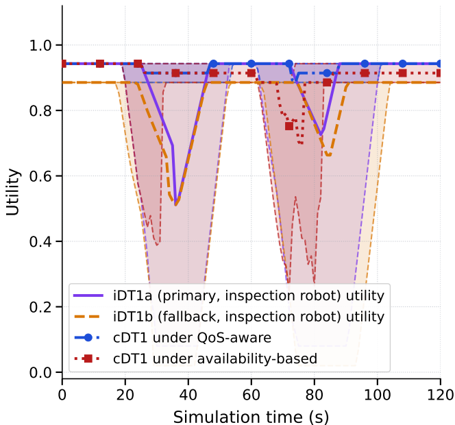
PoC-Grounded (iDT1a vs. iDT1b) — provider utility cascade (iDT degradation → cDT output; shaded p10-p90)
