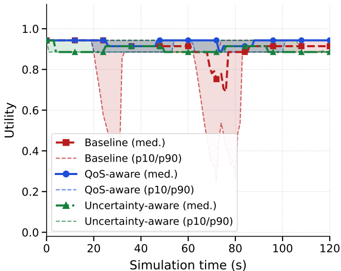
PoC-Grounded (iDT1a vs. iDT1b) — utility over time (30 runs, shaded p10-p90)
