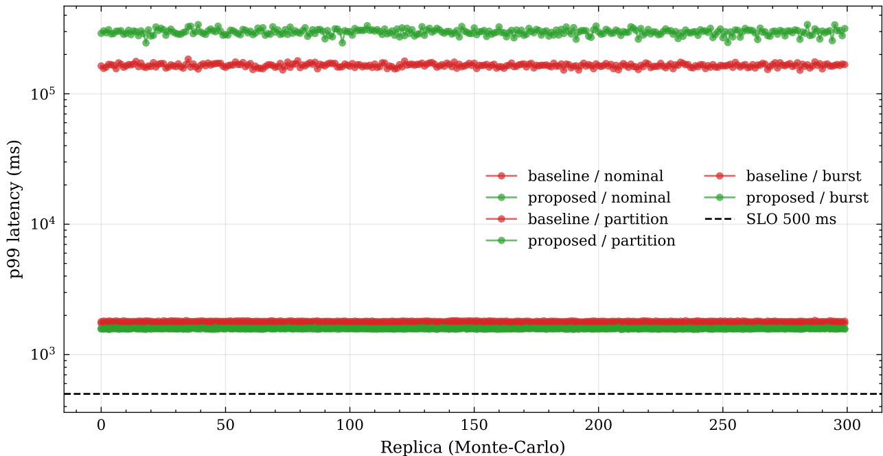
Figure 1 - p99 latency per replica x scenario
