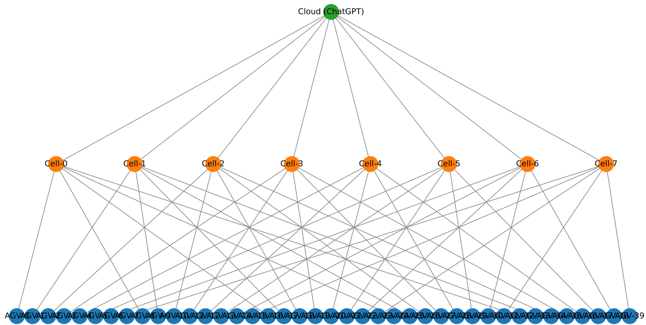
Figure 4 - Mesh topology: 40 AGVs x 8 edge cells x cloud fallback
