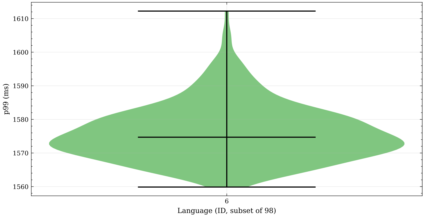
Figure 5 - p99 distribution by language (proposed, nominal)
