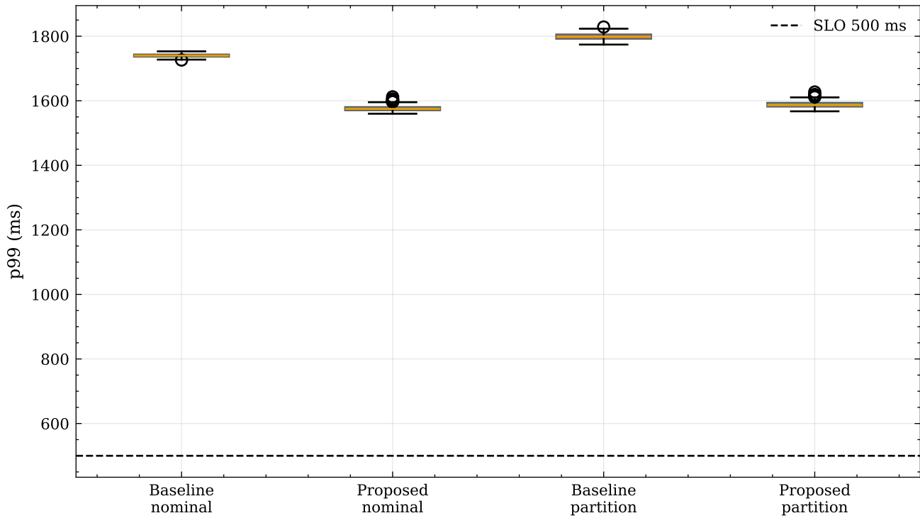
Figure 6 - PACELC: p99 nominal vs partition x arms
