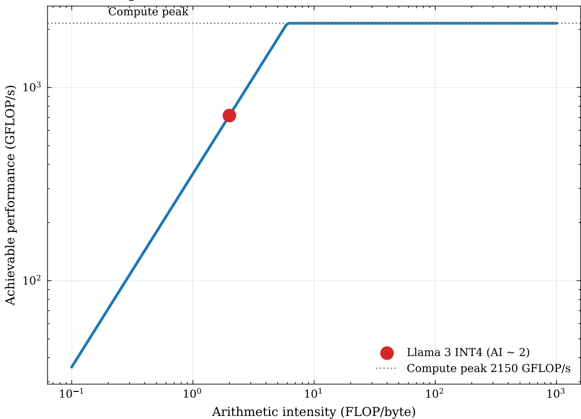
Figure 7 - Roofline Llama 3 INT4 / DDR5-5600 (358 GB/s)
