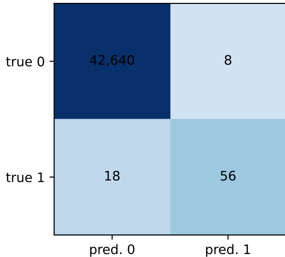
MLP test @ \tau^*=0.9994
