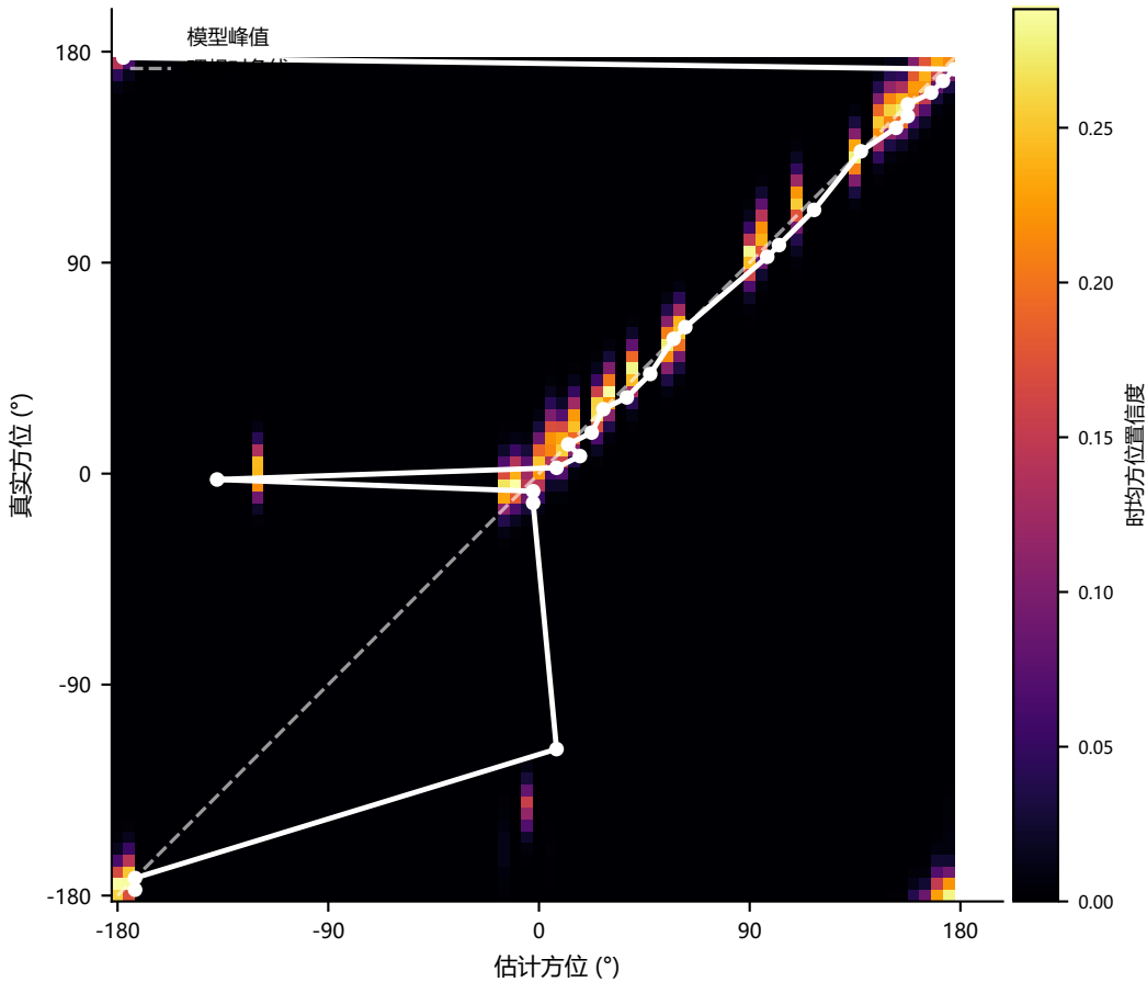
堆叠方位响应场 (stacked DOA field)
