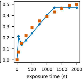
PQ/PMMA, source kinetic model (c) K = 24.94 \text{ rad}/\mu\text{m} , NRMSE 0.10
