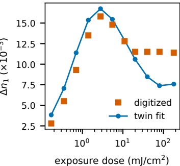
Bayfol HX, source kinetic model (a) K = 8.98 \text{ rad}/\mu\text{m} , NRMSE 0.17
