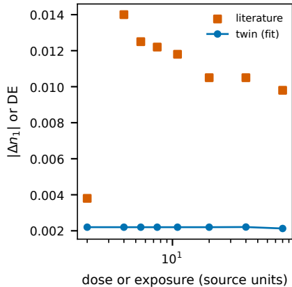
bruder2017_growth_dn_K8.98_exp K=8.98 rad/um NRMSE=0.87 (POOR)
