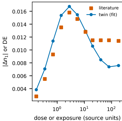
bruder2017_growth_dn_K8.98_sim K=8.98 rad/ \mu m NRMSE=0.17 (GOOD)
