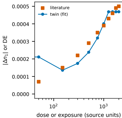
hsieh2022_growth_dn_K24.94 K=24.94 rad/ \mu m NRMSE=0.10 (GOOD)
