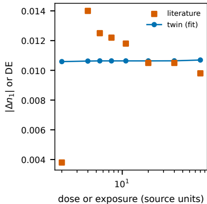
bruder2017_growth_dn_K8.98_exp K=8.98 rad/ \mu m NRMSE=0.28 (GOOD)
