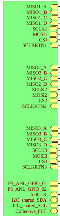
Interface1 Interface Connector.SchDoc
