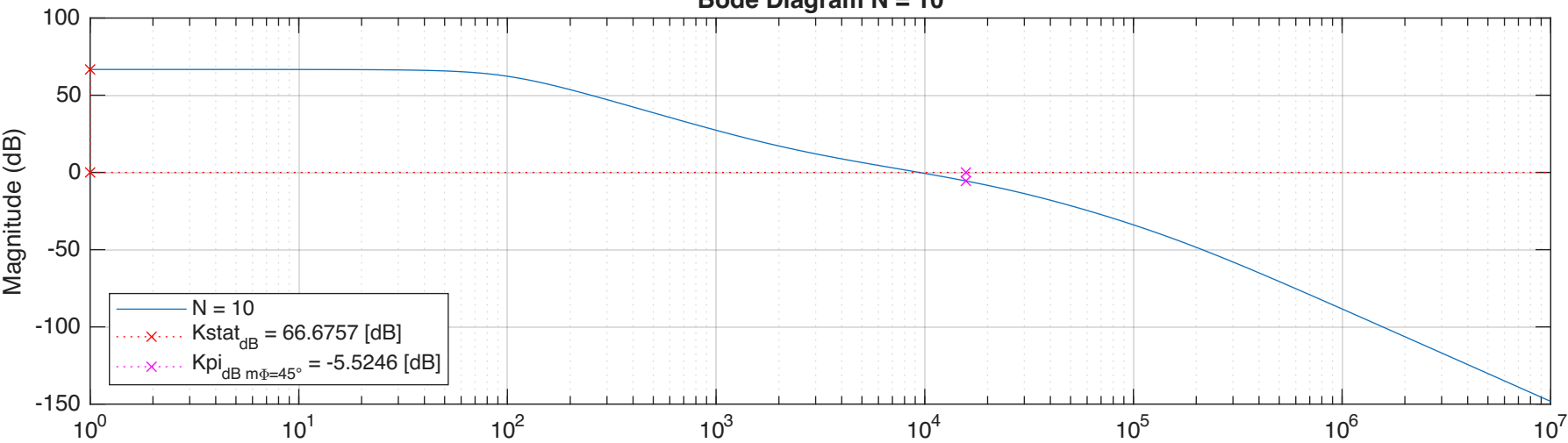
Bode Diagram N = 10
