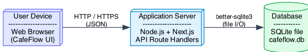
Figure 3.6: Deployment diagram of CafeFlow
