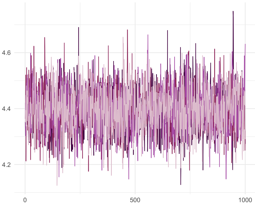
\alpha_0 (Essence of Epiphaneia)
