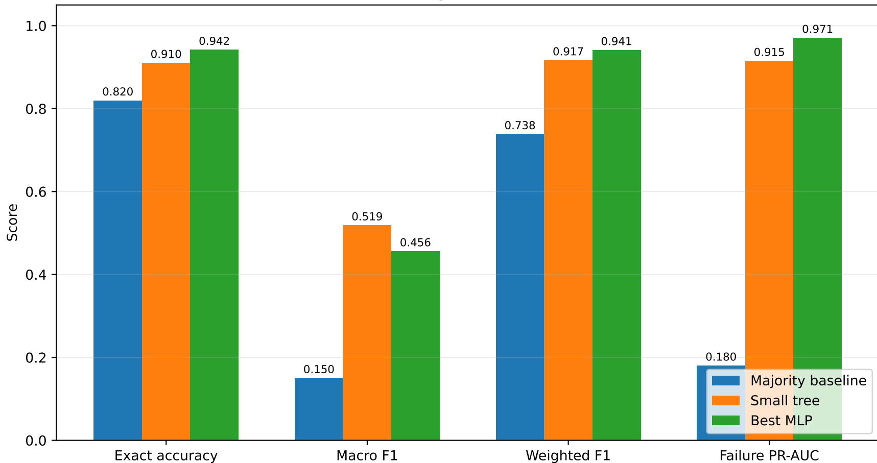
Mission 2512 exit-flag models — held-out frames
