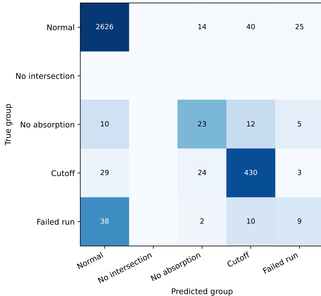
Small depth-8 tree
