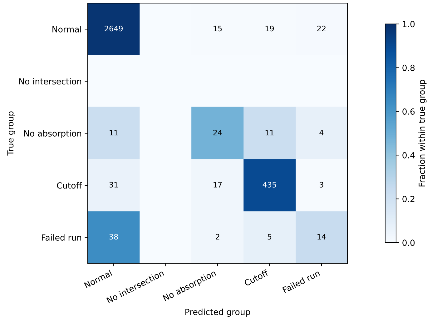
Best profile MLP
