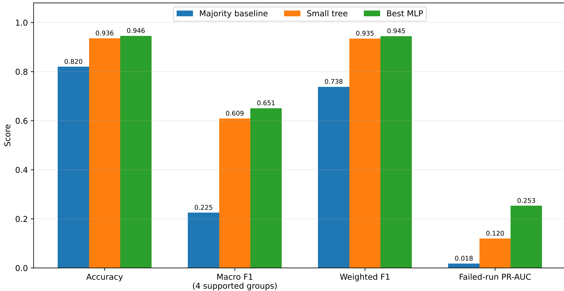
Grouped exit-flag models — held-out comparison
