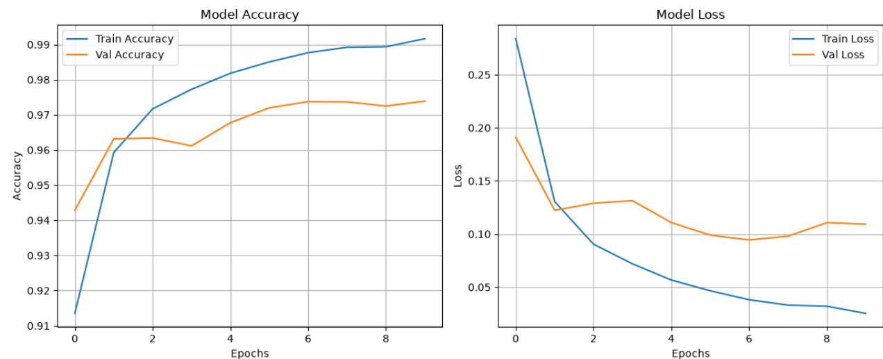
Layers (512, 128, 32) , Act: ELU , No Drop-Out
