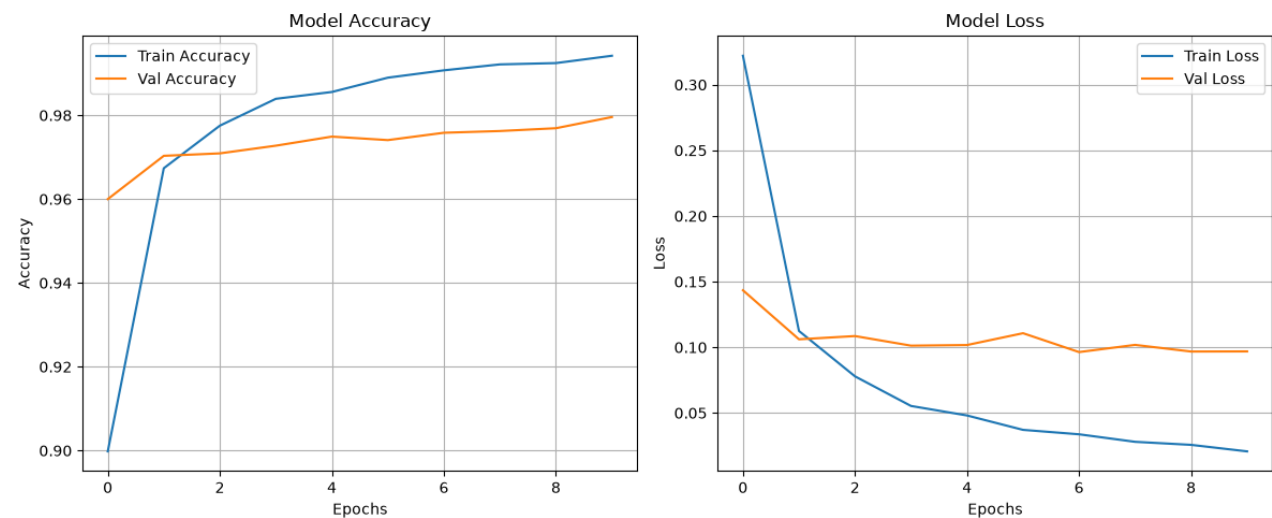
Layers (512, 256, 128, 64, 32) , Act: GELU , No Drop-Out
