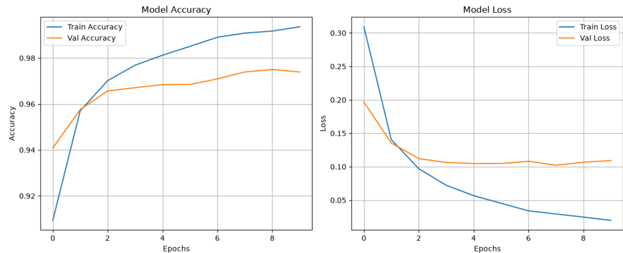
Layers (128, 64), Act: ELU , No Drop-Out
