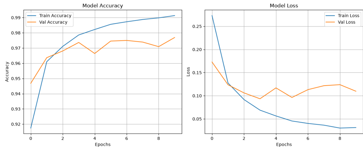
Layers (512, 256) , Act: ELU , No Drop-Out
