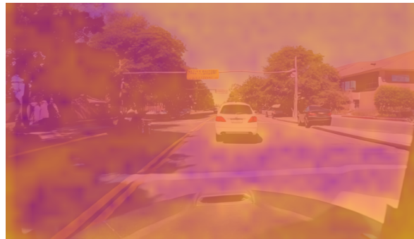
+ Saliency (step 40)
