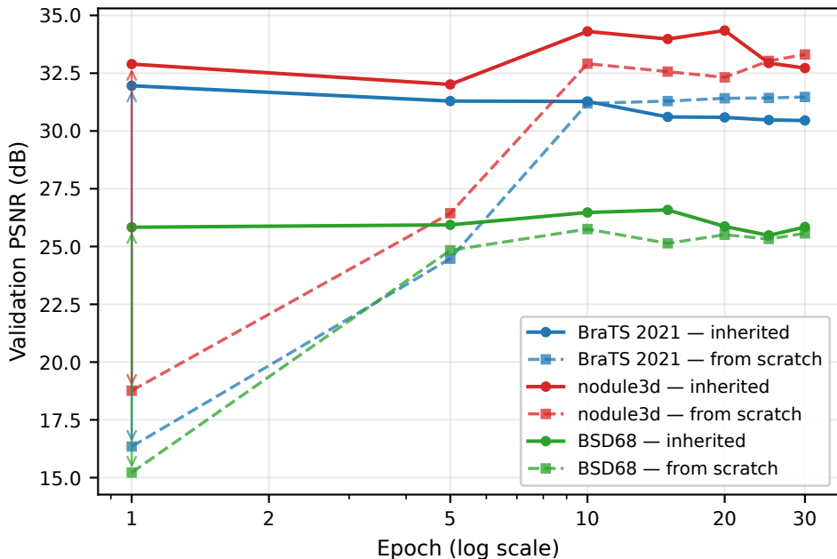
Weight inheritance vs. from-scratch training (agent 2)
