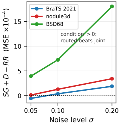
(b) Theorem 2.4 condition
