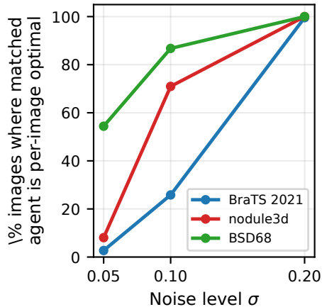
(c) Why routing regret vanishes
