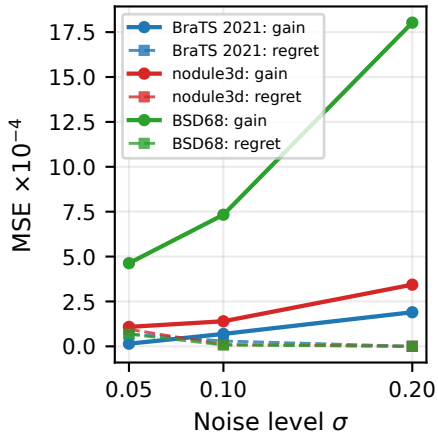
(a) Specialisation gain vs. routing regret
