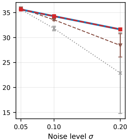
nodule3d
