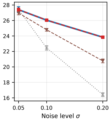
BSD68
