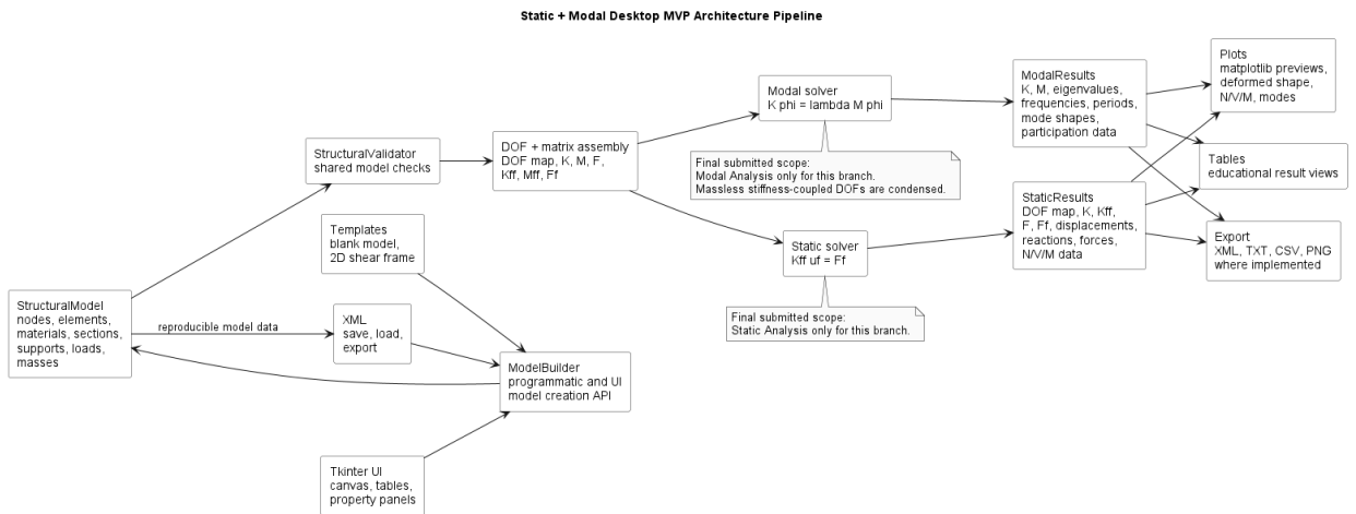
Figure 2: Architecture pipeline
