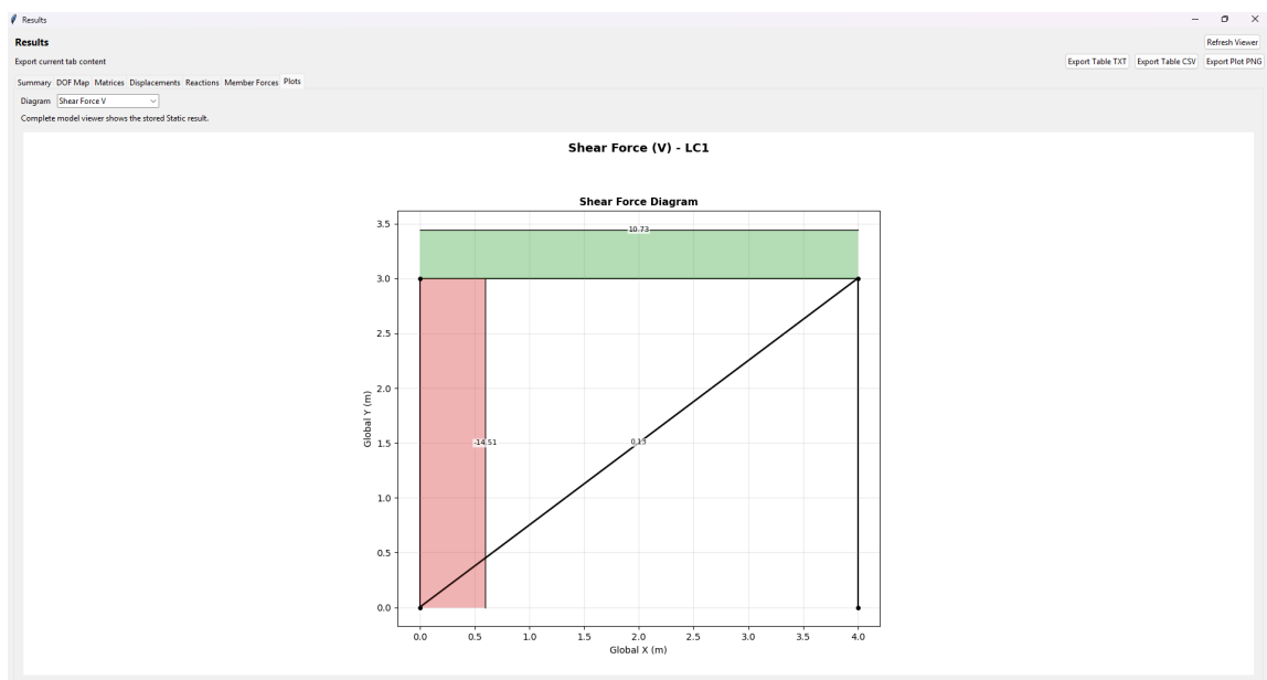
Figure 19: Static frame shear force diagram.
