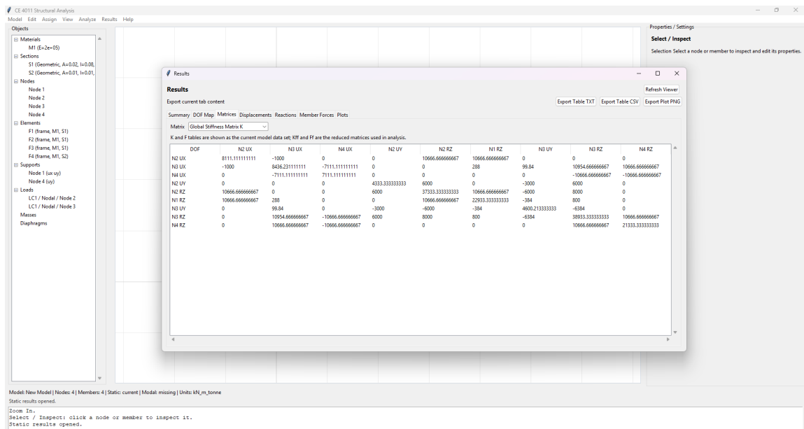
Figure 21: Static frame stiffness matrix K .
