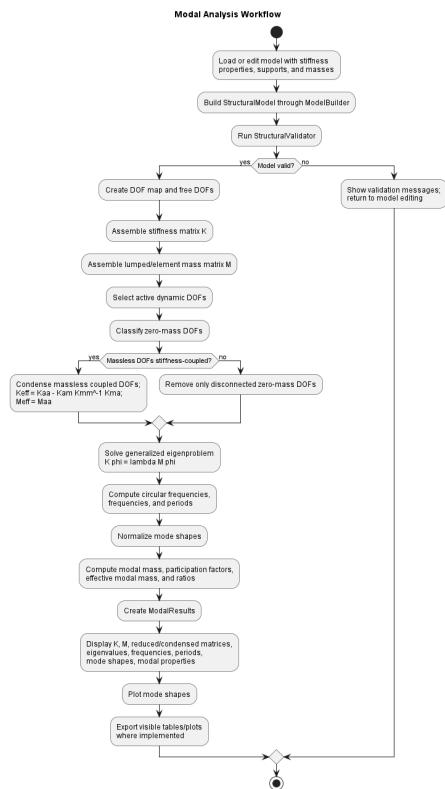
Figure 23: Modal analysis workflow
