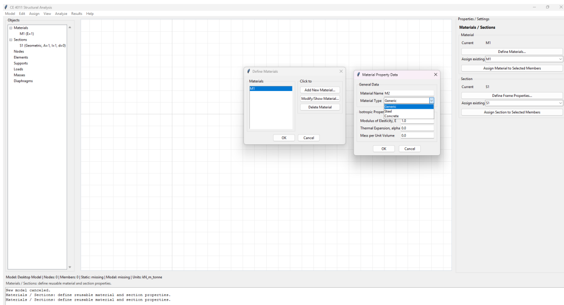
Figure 8: Property panel
