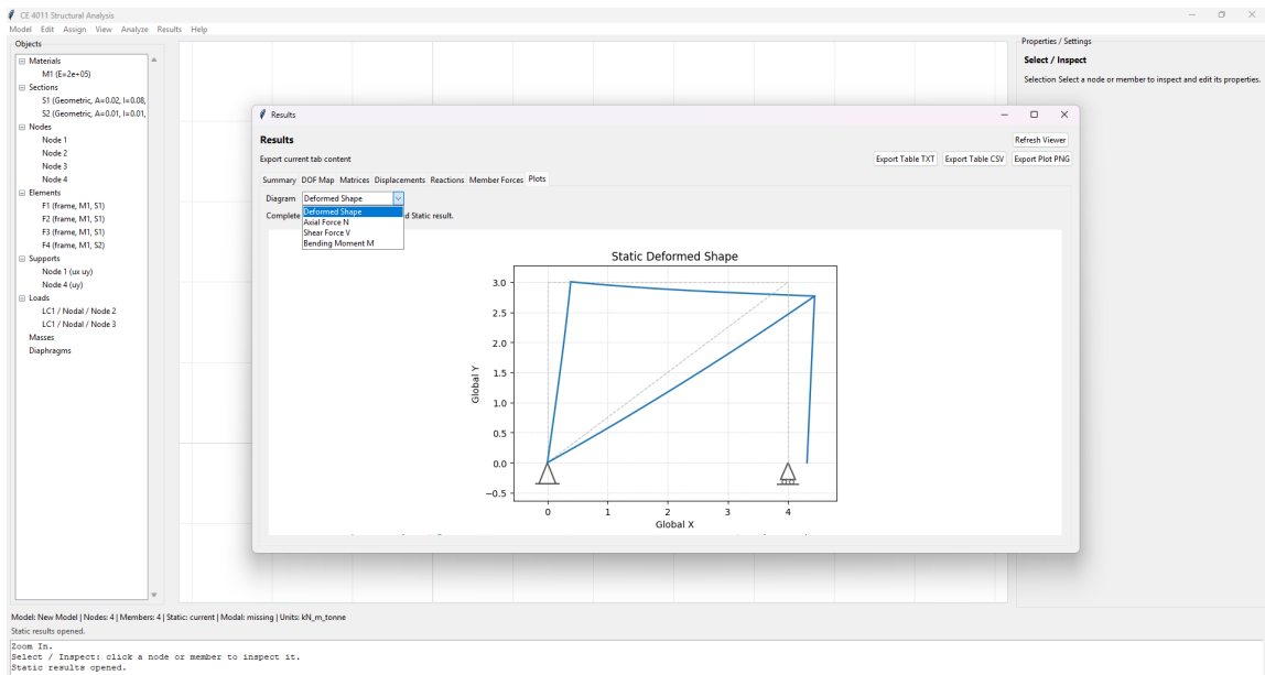
Figure 17: Static deformed shape
