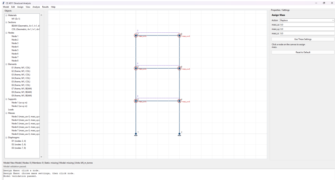
Figure 13: Validation status/dialog
