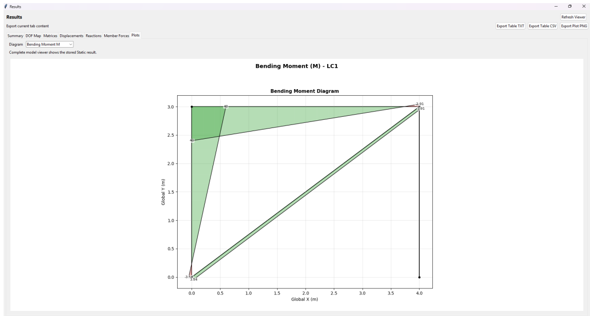
Figure 20: Static frame bending moment diagram.
