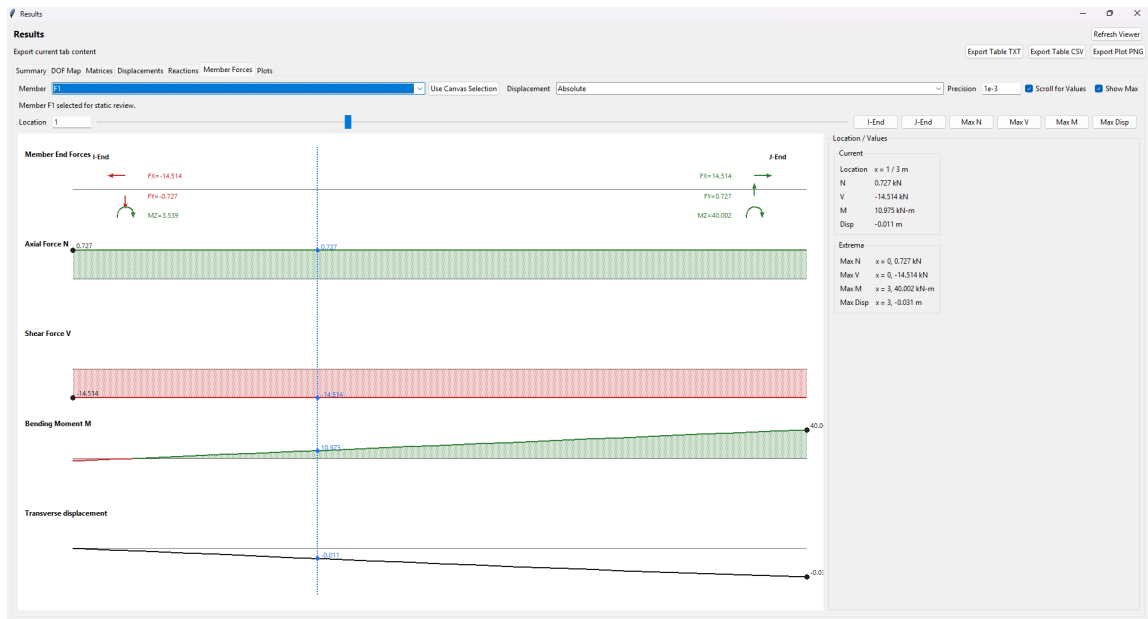
Figure 22: Static frame individual member result plot.
