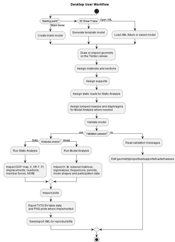
Figure 1: Desktop workflow
