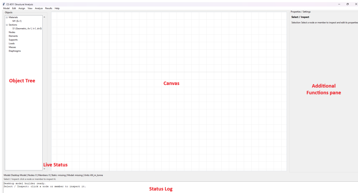
Figure 7: Model canvas
