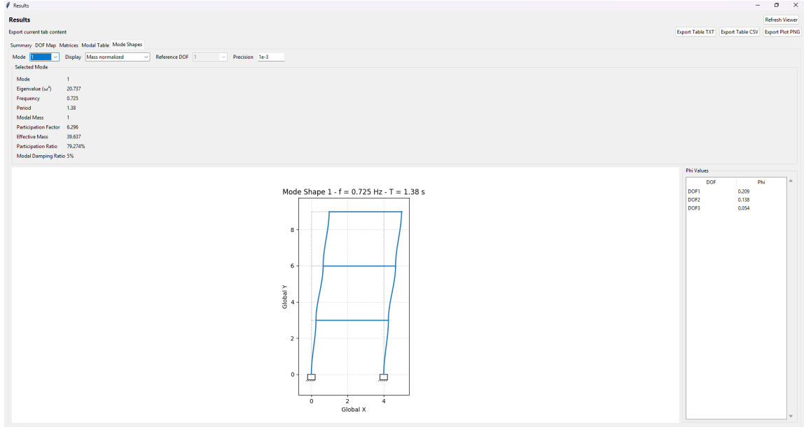
Figure 28: Mode shape plot
