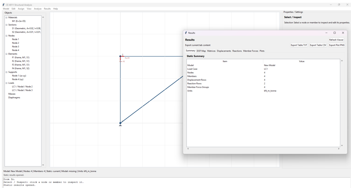
Figure 15: Static result summary
