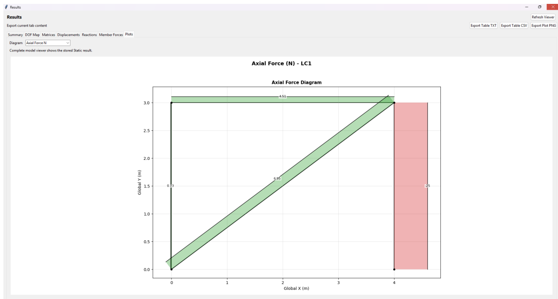
Figure 18: Static frame axial force diagram.
