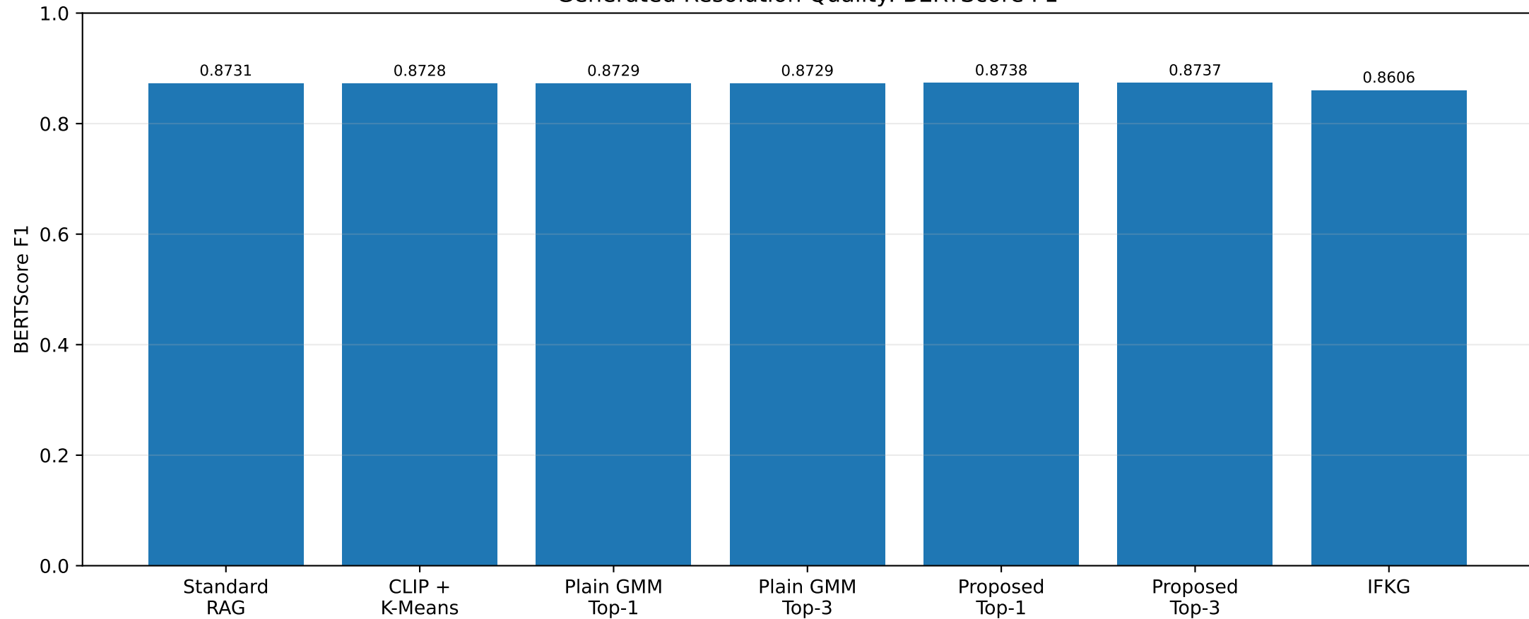
Generated Resolution Quality: BERTScore F1
