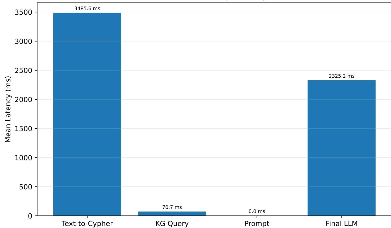
IFKG Inference Latency Decomposition
