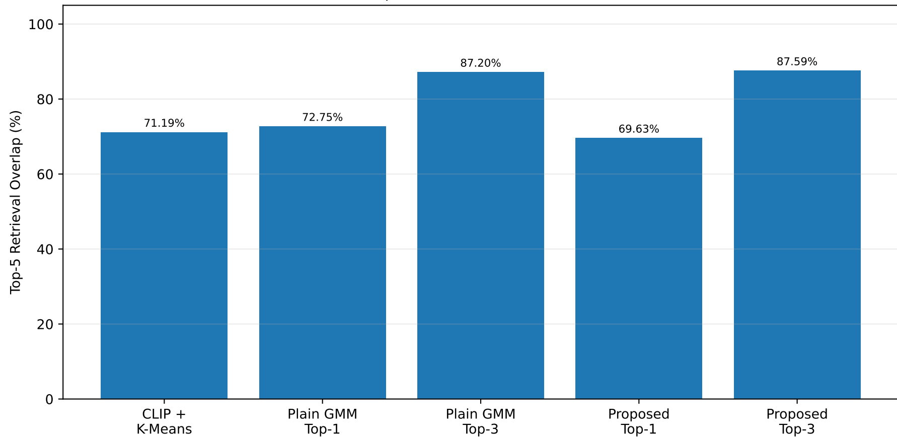
Top-5 Retrieval Preservation
