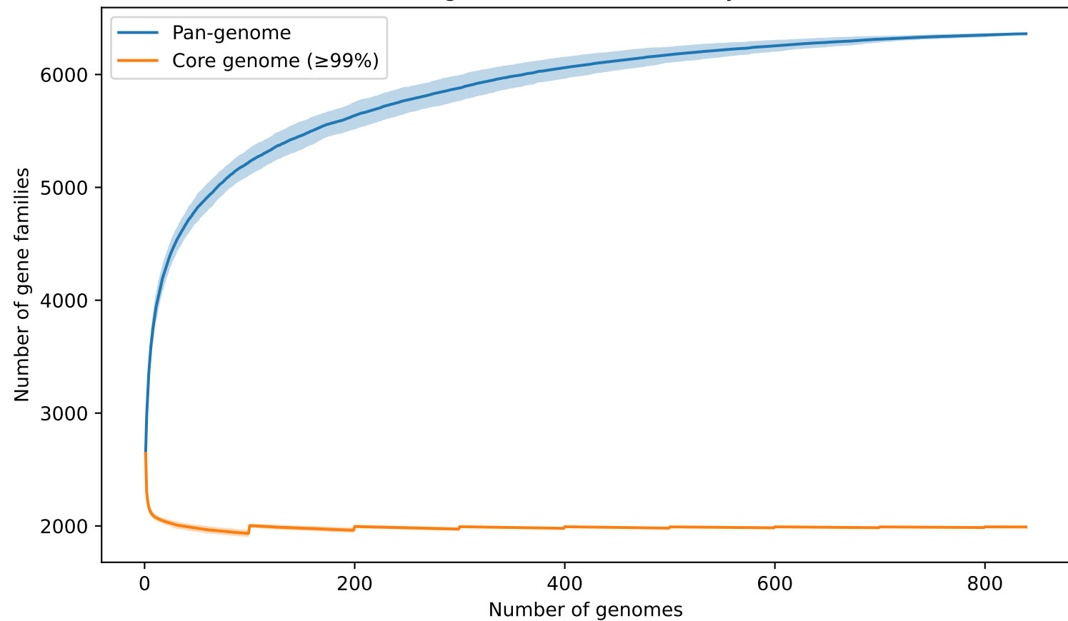
Pangenome rarefaction analysis
