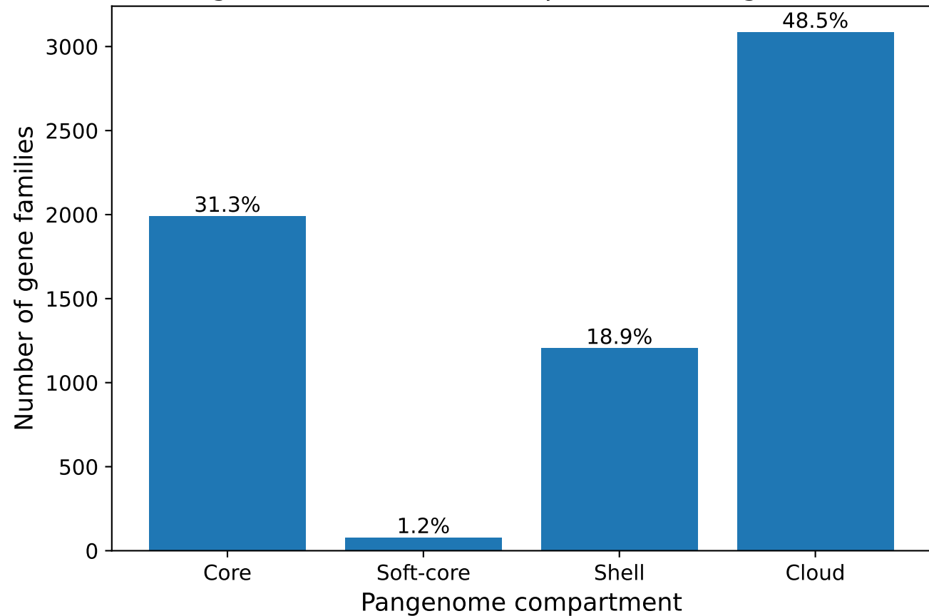
Pangenome structural composition (839 genomes)
