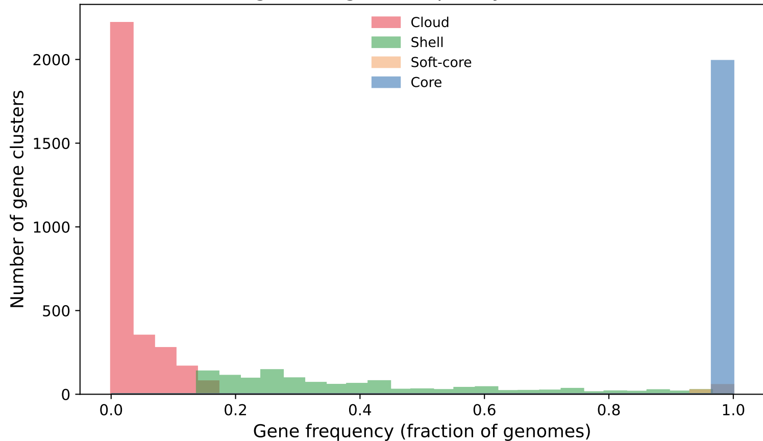
Pangenome gene frequency distribution
