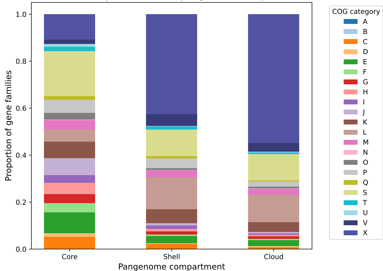
Functional composition across pangenome compartments
