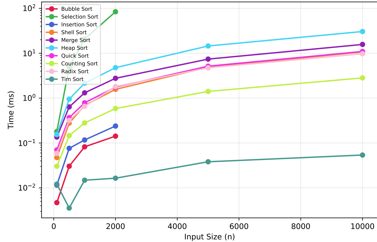
Nearly Sorted
