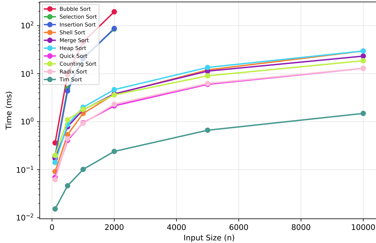
Reverse Sorted
