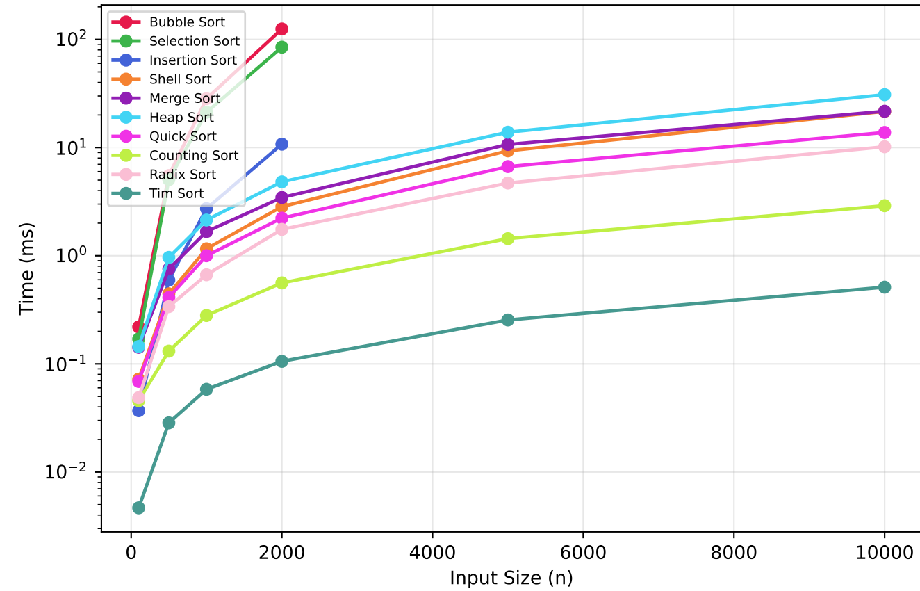
Nearly Sorted
