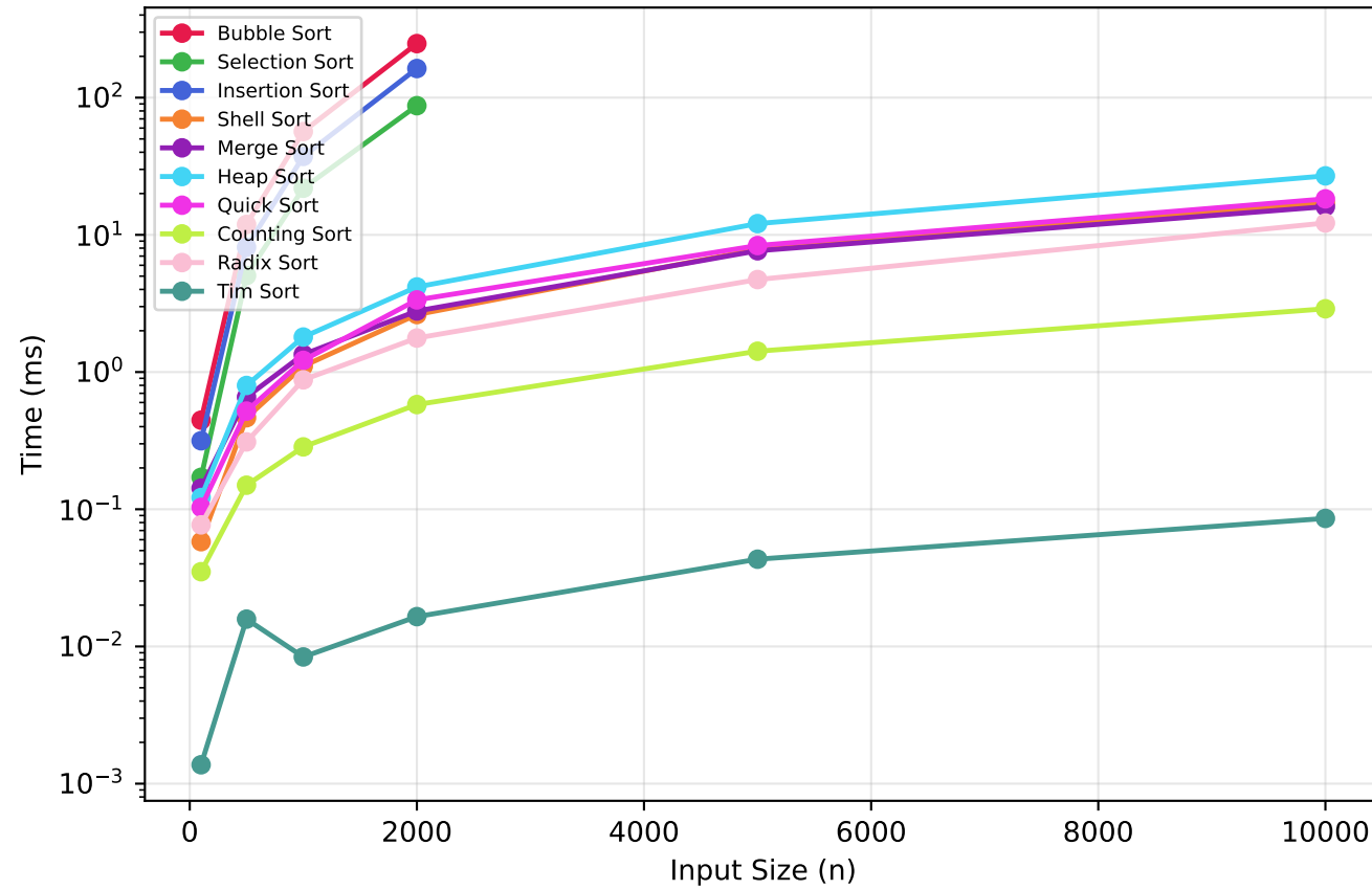
Reverse Sorted
