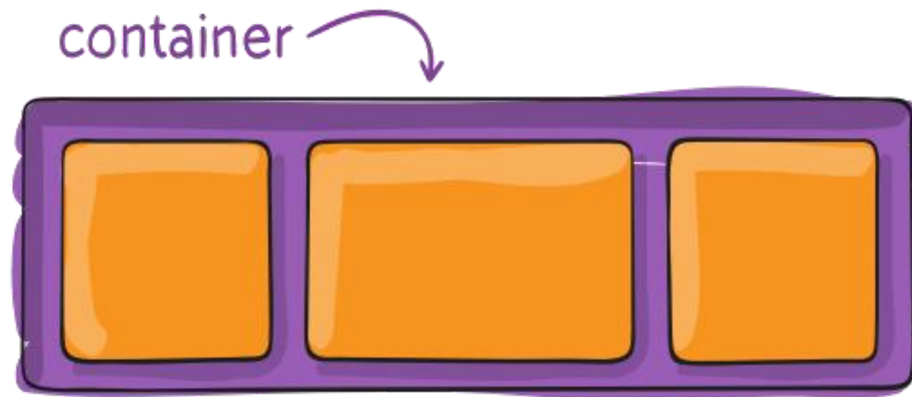
Flex Container
