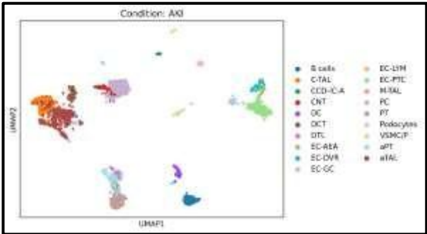
UMAP by condition
