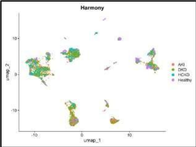
Harmony condition
