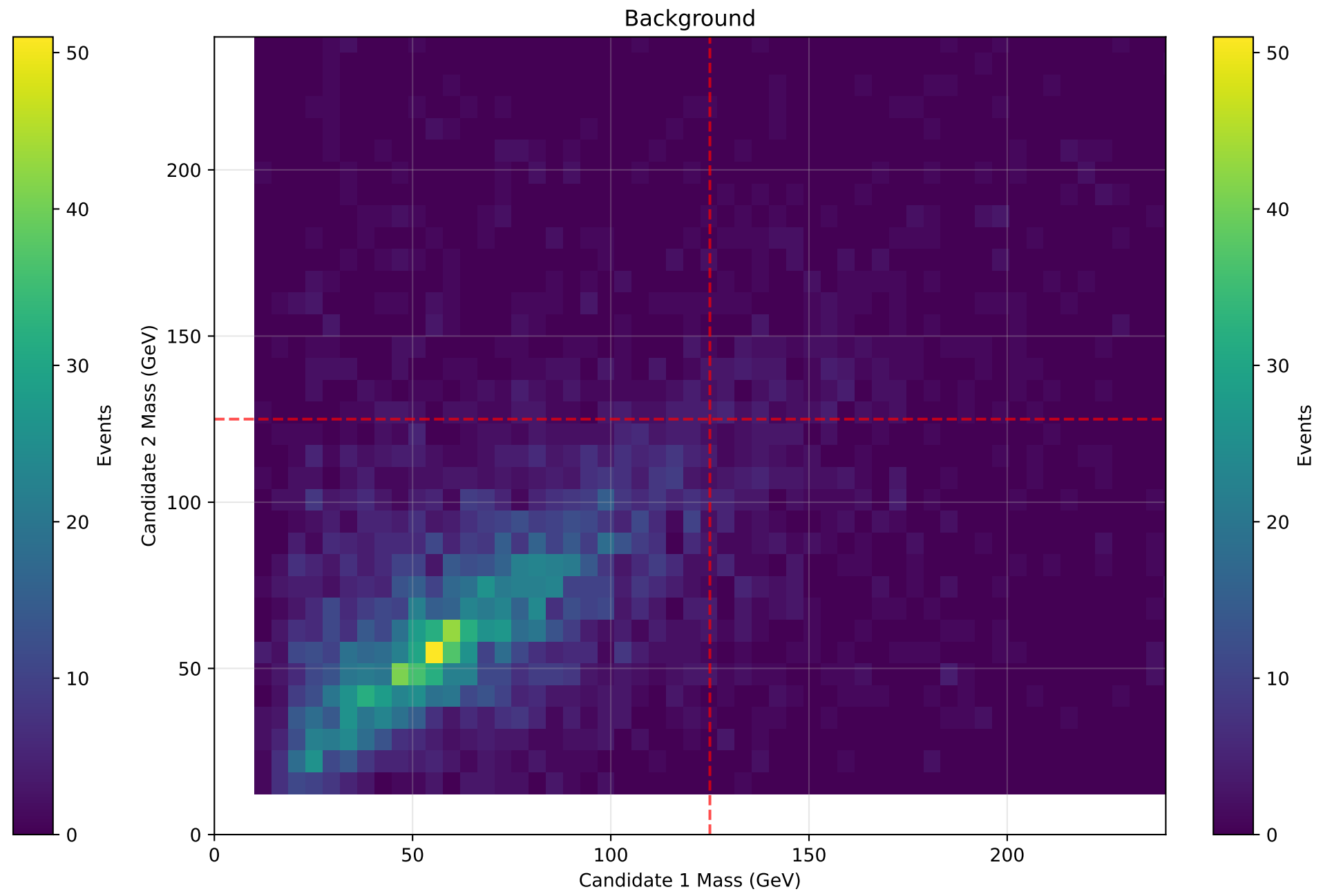
2D Histogram of Higgs Candidate Masses (Signal vs Background)
