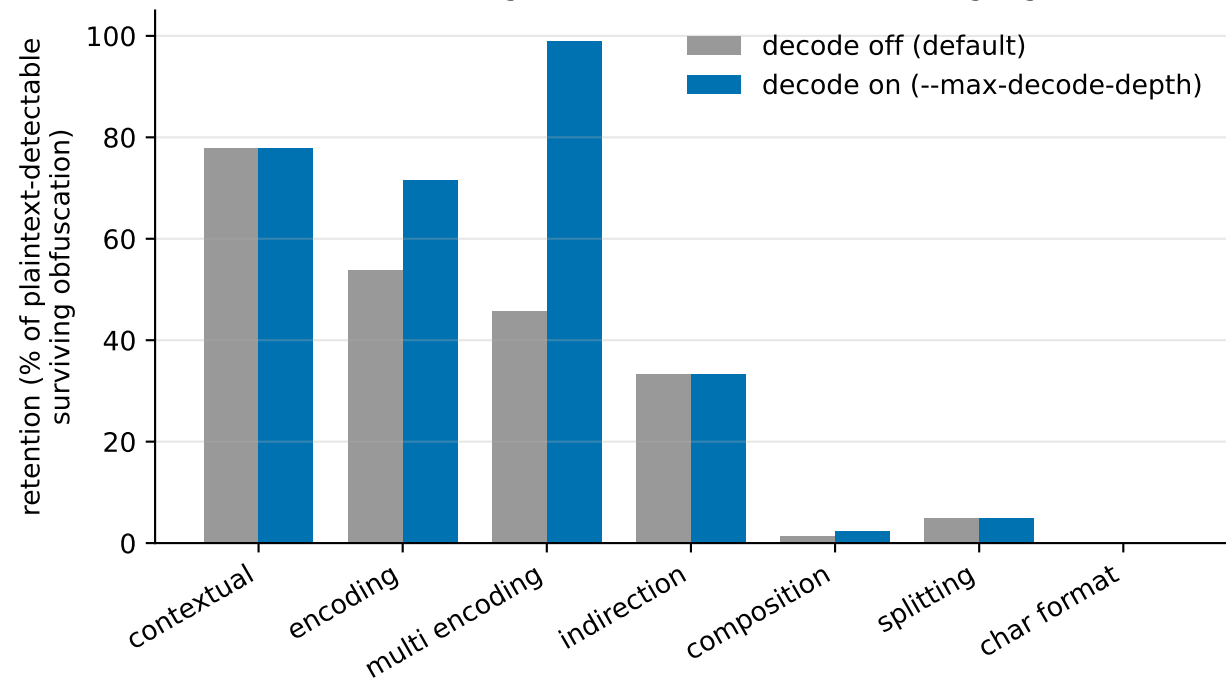
Recursive decoding recovers Base64/Hex encodings (gitleaks)
