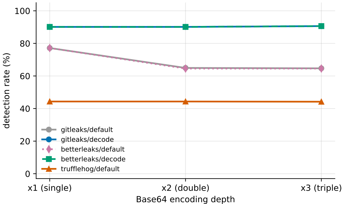
Detection vs multi-encoding depth
