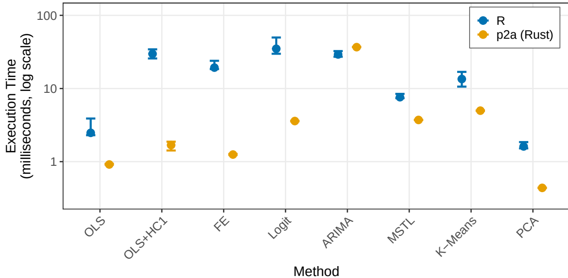
Figure 1: Comparison of execution times between R reference implementations (blue) and prompt2analytics (orange). All benchmarks use n = 10,000 observations. Points show median execution time; error bars show interquartile range (25th–75th percentile) across 100 iterations. The y-axis uses a logarithmic scale.
