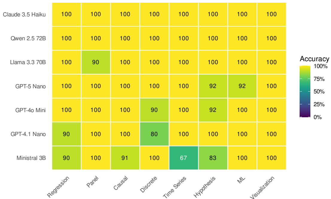
Figure 10: Accuracy breakdown by test category. Darker cells indicate lower accuracy. Most models achieve 100% on standard categories; errors concentrate in edge cases involving ambiguous method selection (e.g., logit with fixed effects vs. FEGLM).
