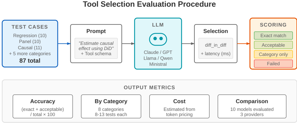
Figure 8: Tool selection evaluation procedure. Each of 87 test cases presents a natural language prompt describing an analytical task. The LLM receives the prompt along with the prompt2analytics tool schema and must select the appropriate method. Responses are scored by comparing the selected tool against expected answers.
