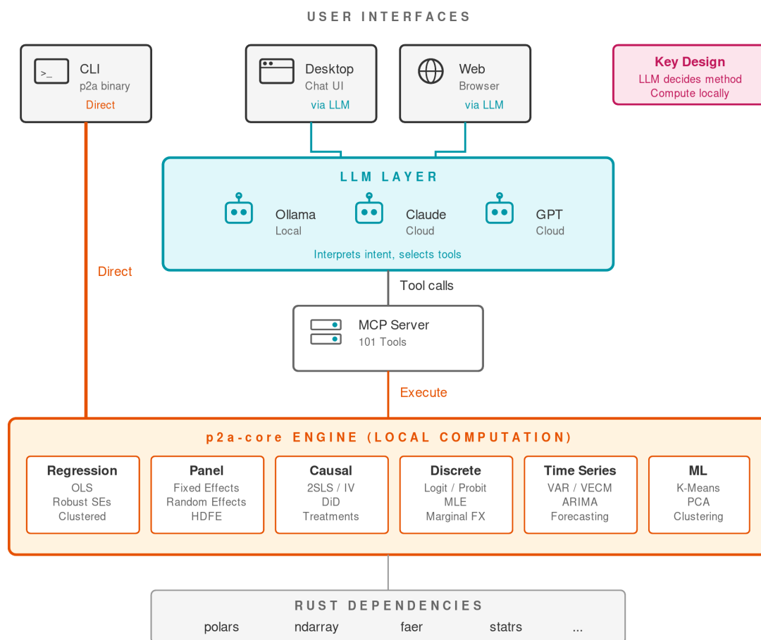
Figure 1: Software architecture of prompt2analytics . The CLI accesses the analytics engine directly (orange); chat interfaces route through the LLM layer and MCP server (cyan). All computation occurs locally in p2a-core .
