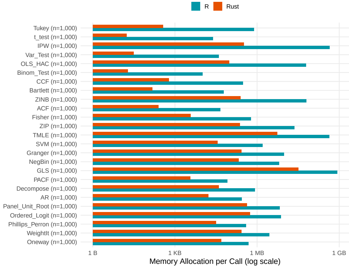
Figure 5: Memory allocation comparison between R and Rust implementations by method category. Rust consistently allocates less memory, with the largest savings in panel data and treatment effect methods.
