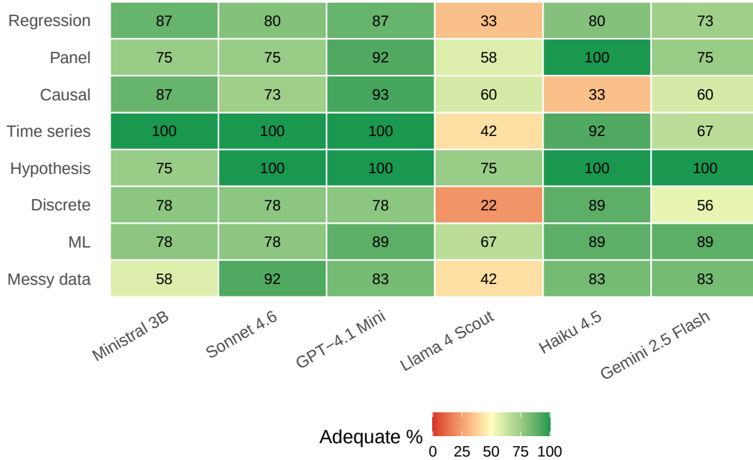
Figure 3: Adequate rate by test category and model (red = low, green = high). Errors concentrate in ambiguous method selection (causal inference, discrete choice).
