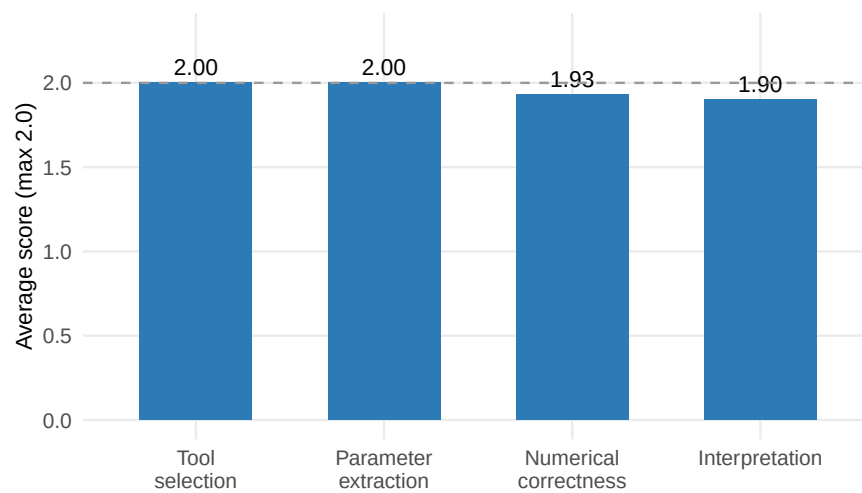
Figure I.2: Per-dimension scoring averages across 30 turns (Claude Sonnet 4.6, Chrome evaluation).
