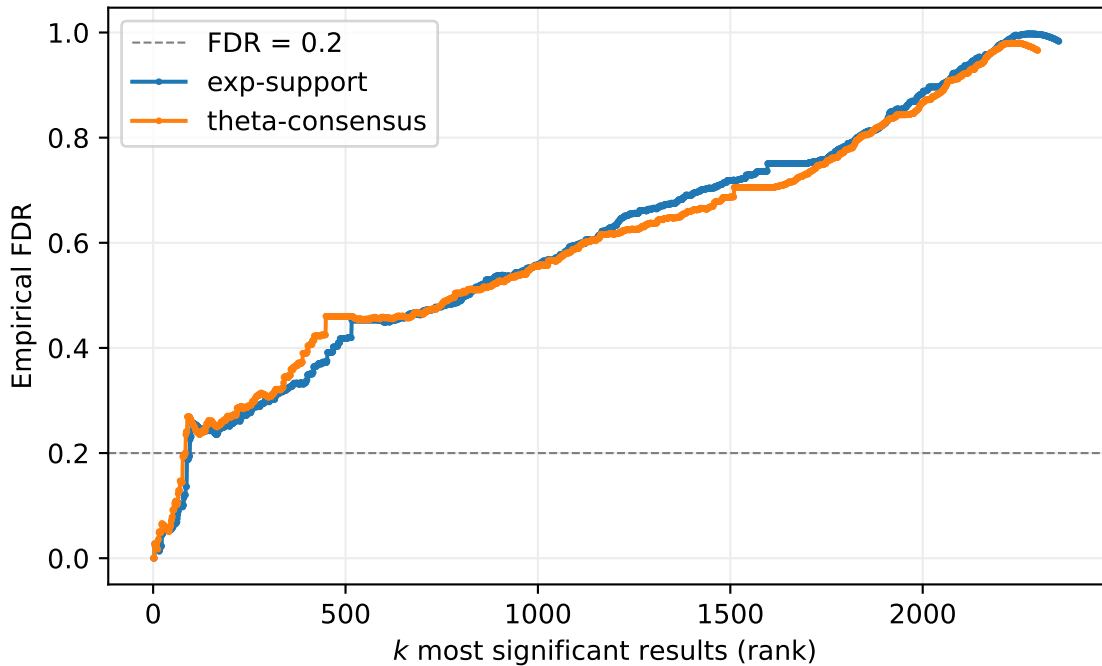
breastCancer sigma=2 theta=1.0
