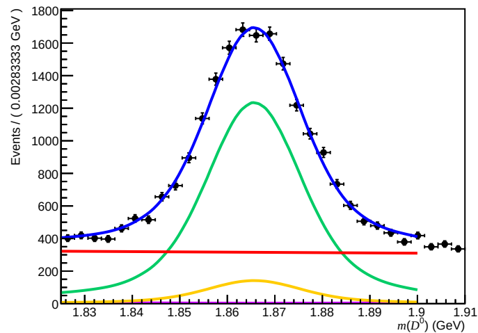
Passed ( 0 < n_{\text{Tracks}} < 200 , 3.6 < \eta < 5.0 , 60000 < p < 100000 )
