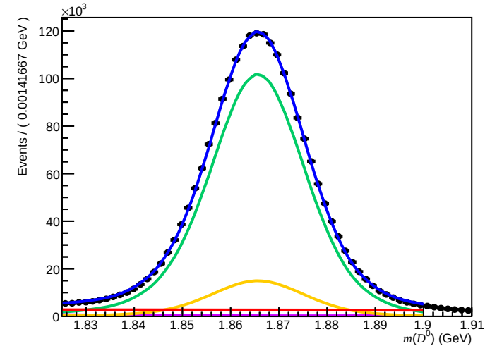
Failed ( 0 < n_{\text{Tracks}} < 200 , 3.6 < \eta < 5.0 , 60000 < p < 100000 )
