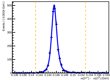
Passed DiF (after RICH1) ( 200 < nTracks < 600 , 1.7 < \eta < 3.6 , 3000 < p < 6000 )
