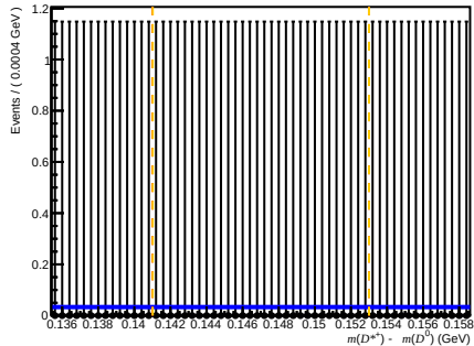
Passed DiF (before RICH1) ( 200 < nTracks < 600 , 1.7 < \eta < 3.6 , 3000 < p < 6000 )
