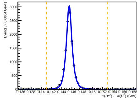
Failed DiF ( 200 < nTracks < 600 , 1.7 < \eta < 3.6 , 3000 < p < 6000 )
