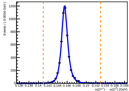
Passed DIF (after RICH1) ( 200 < nTracks < 600 , 1.7 < \eta < 3.6 , 6000 < p < 10000 )
