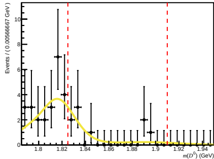
Total ( 200 < n\text{Tracks} < 600 , 3.6 < \eta < 5.0 , 10000 < p < 15600 )
